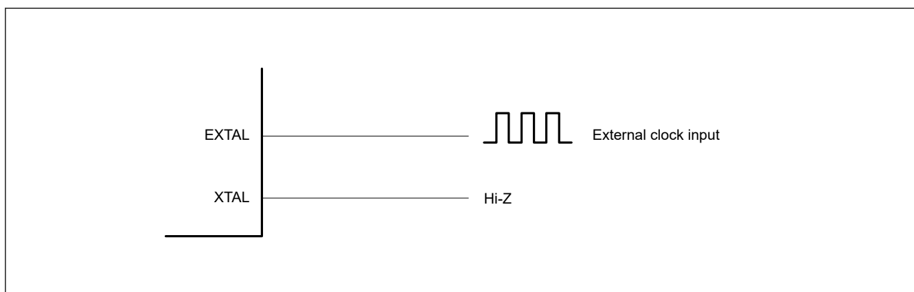
Figure 9.4 Equivalent circuit for external clock
